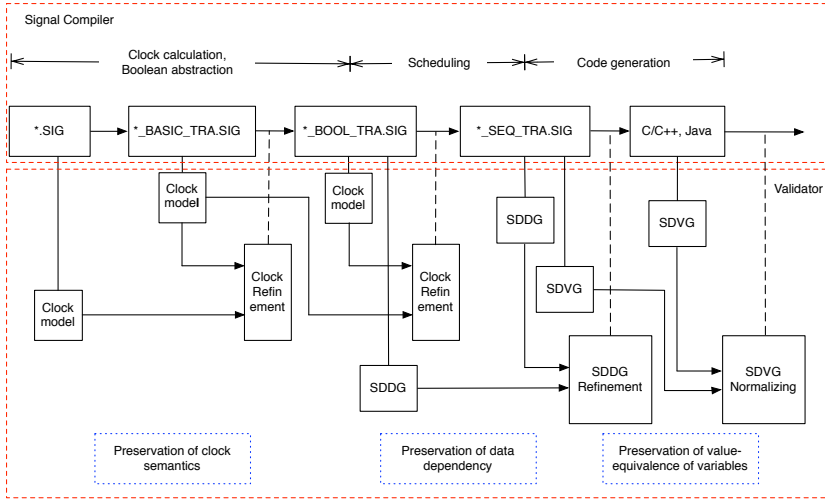
Fig. 1 Translation validation for the Signal compiler
