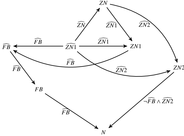
Fig. 5 The SDDG of DEC
