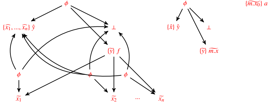
Fig. 9 The graphs of y := f(x_1, \dots, x_n) and y := x \text{! init } a
