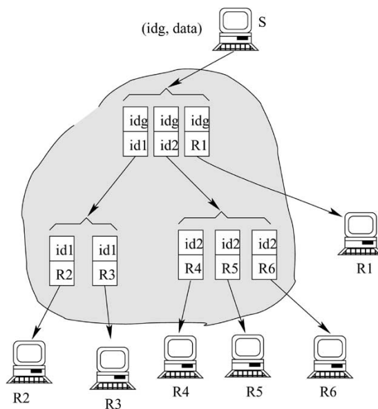
Fig. 5. Example of a scalable multicast tree with bounded degree by using chains of triggers.
