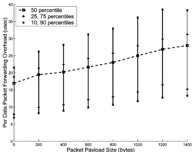
Fig. 10. Per packet forwarding overhead as a function of payload packet size. In this case, the i3 header sizes 48 bytes.
