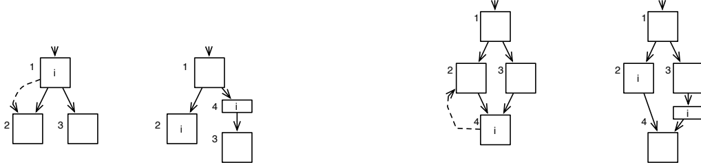
Figure 1. The two extra rules of trace scheduling. On the left, an example of move after a condition. On the right, an example of move before a join point. On each example the code is shown before and after hijacking.
