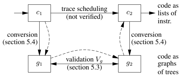
Figure 2. Overview of trace scheduling and its validation. Solid arrows represent code transformations and validations. Dashed arrows represent proofs of semantic preservation.
