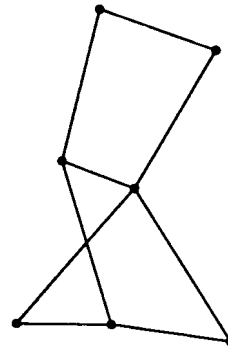
Figure 35. Graph in Figure 6(c) from Eades 3
