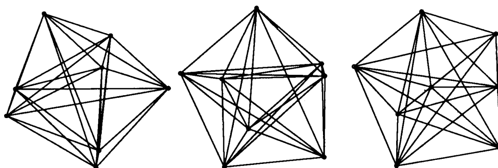
Figure 68. Three-dimensional layouts of K_6
