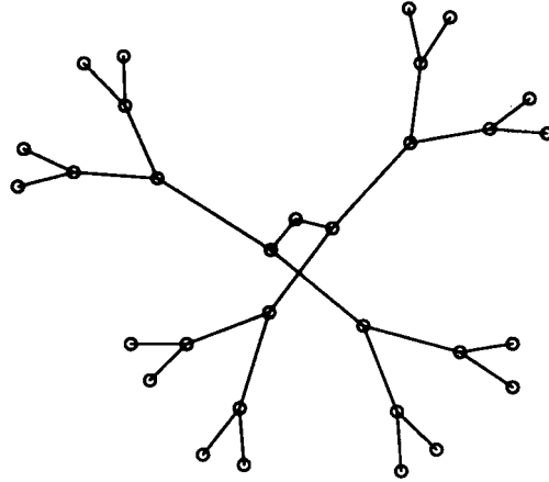
Figure 41. Tangled binary tree (graph in Figure 14(a) from Davidson and Harel 10 )
