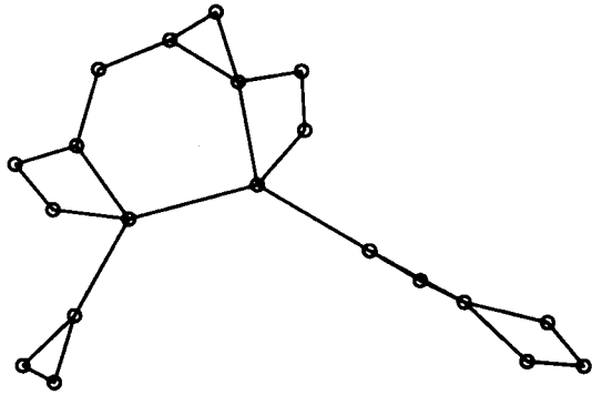
Figure 75. Graph in Figure 6(a) from Eades 3
