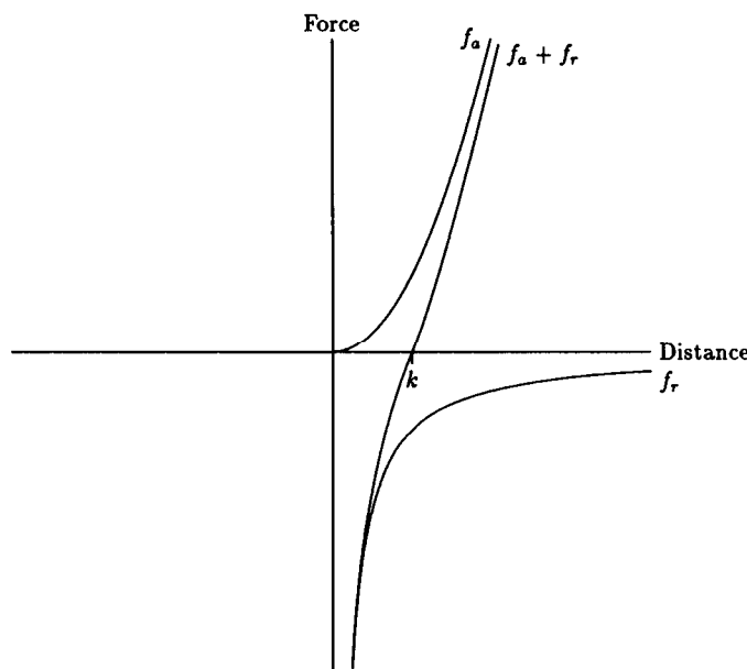
Figure 2. Forces versus distance
